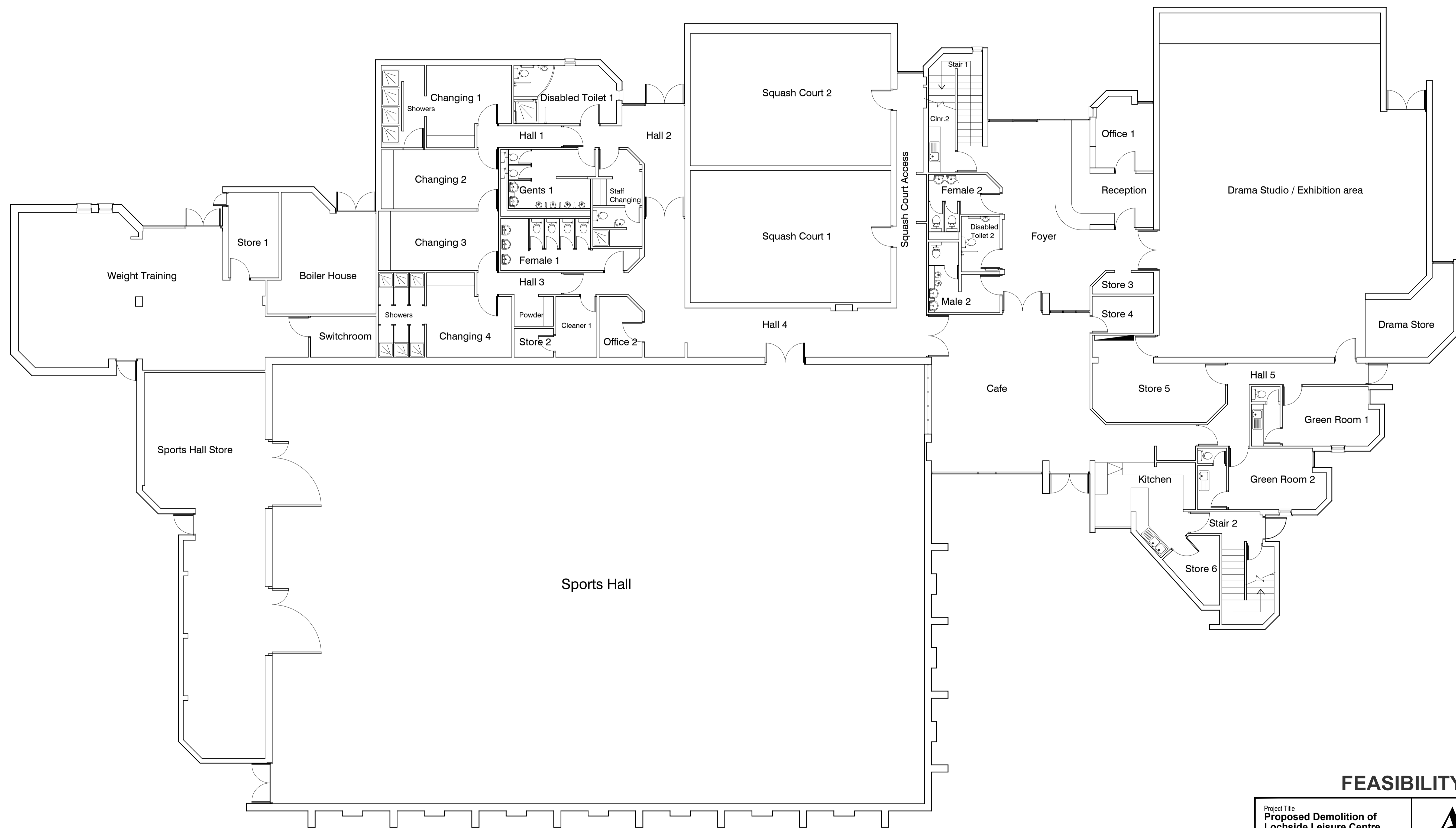
Ground Floor Plan as Existing Scale 1:100 0 1 2 3 4 5 metres
